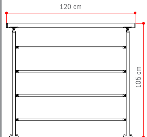
BACK BALUSTRADE K04114000
